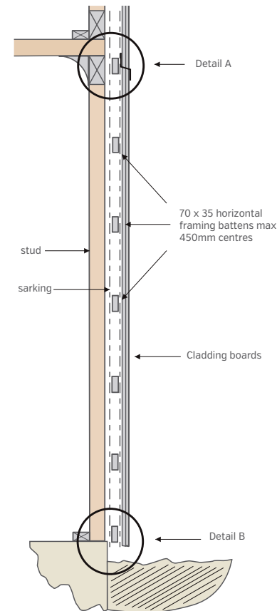
Stud Frame Detail Typical vertical installation
