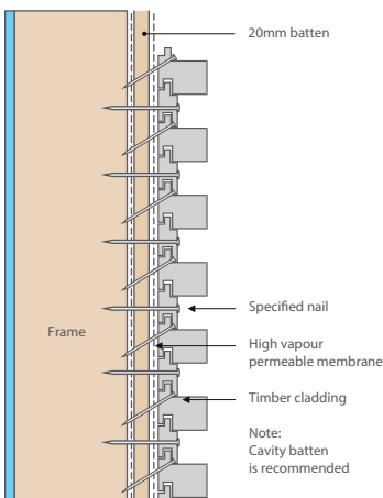
Horizontal installations – external
