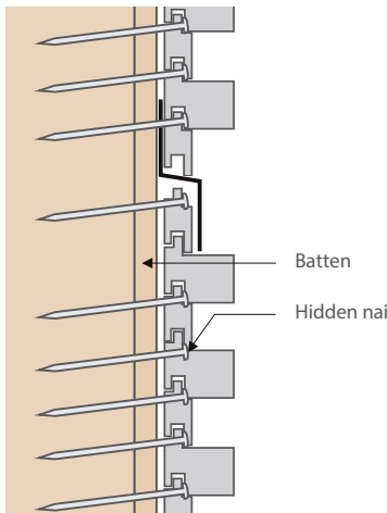
Horizontal installation – internal wall
