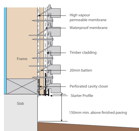
Minimum clearance of cladding above final ground levels and finishing below bottom plate
