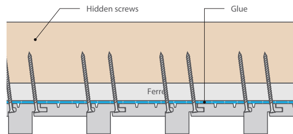
Horizontal installation – internal ceiling
