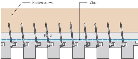
Horizontal installation – internal ceiling
