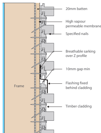
Expansion gap located at every storey
