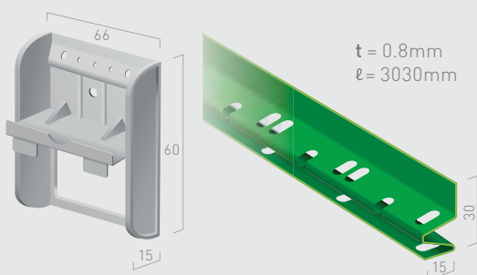
Panel Clip
