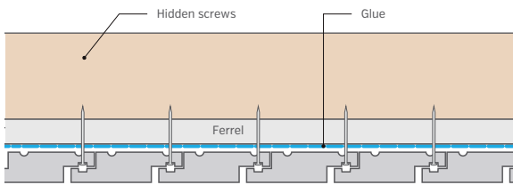
Horizontal installation - internal ceiling
