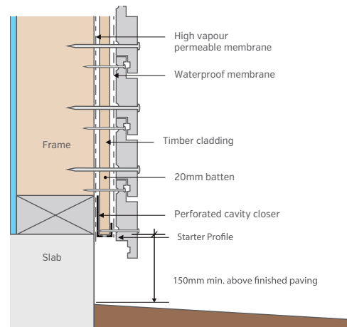
Minimum clearance level of cladding above final ground levels and finishing below bottom plate
