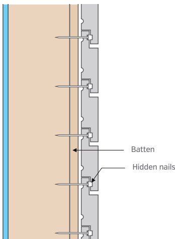
Horizontal installation - internal wall
