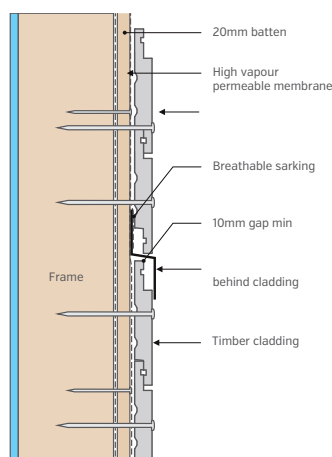
Face fixing showing fixing position
