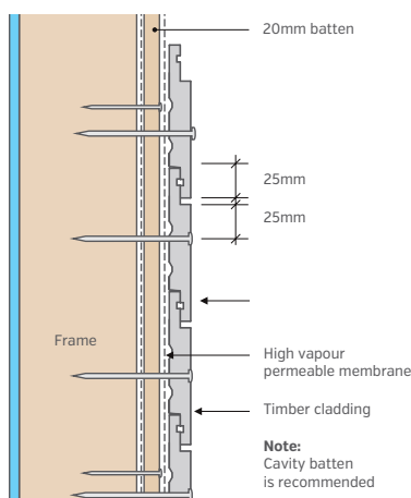
Horizontal installation - external
