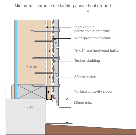
Minimum clearance level of cladding above final ground levels and finishing below bottom plate
