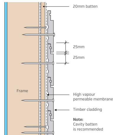
Face fixing showing fixing position
