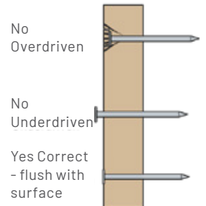
Figure 3: Nail Driving detail
