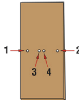
Figure 2: Wide Shingle Fastener detail
